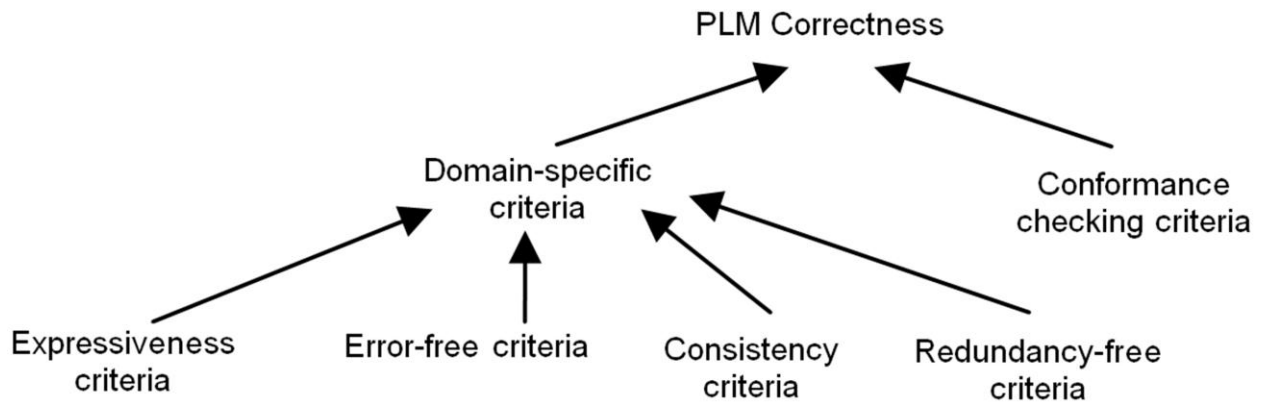
Figure 3. Typology of verification criteria on PLMs
