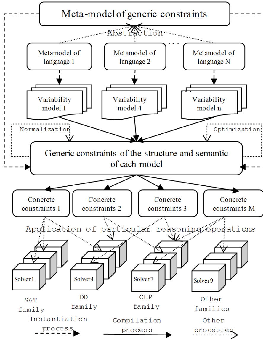
Figure 2. Generic constraints to represent variability models.
